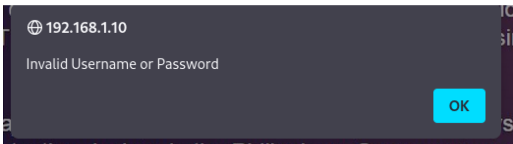
Figure 34 Incorrect password
