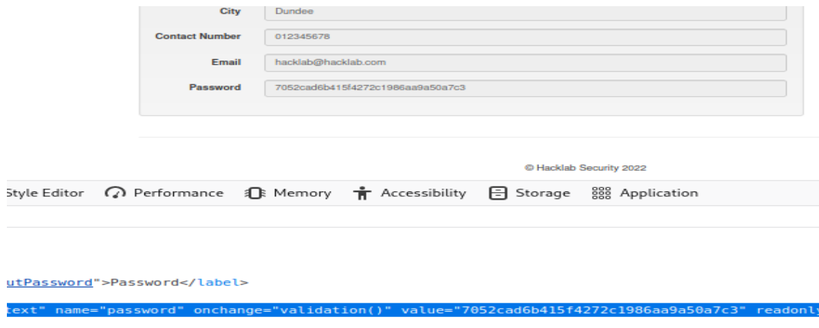
Figure 43 Password Hashing
