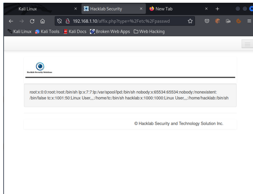
Figure 45 'etc/passwd' file
