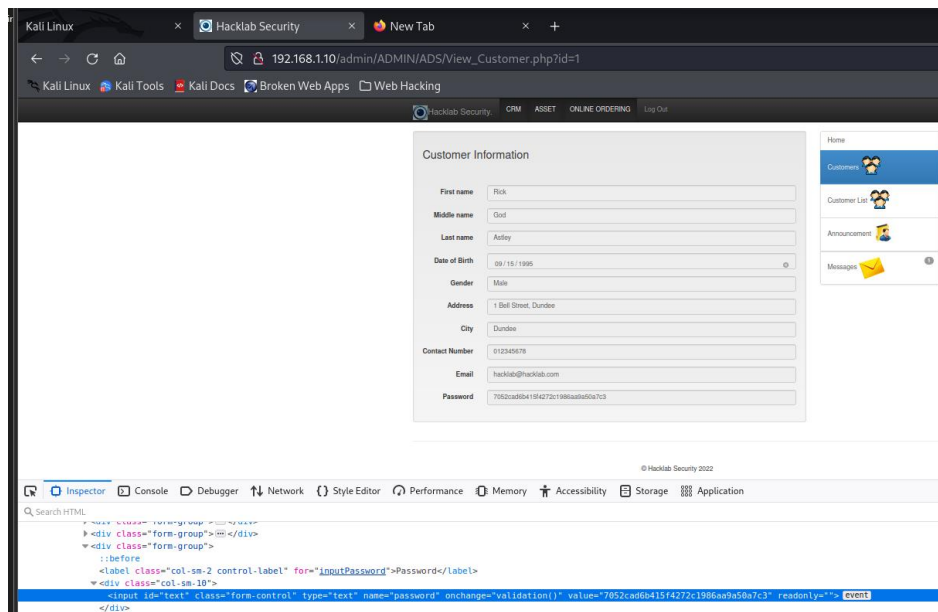
Figure 26 Customer Information
