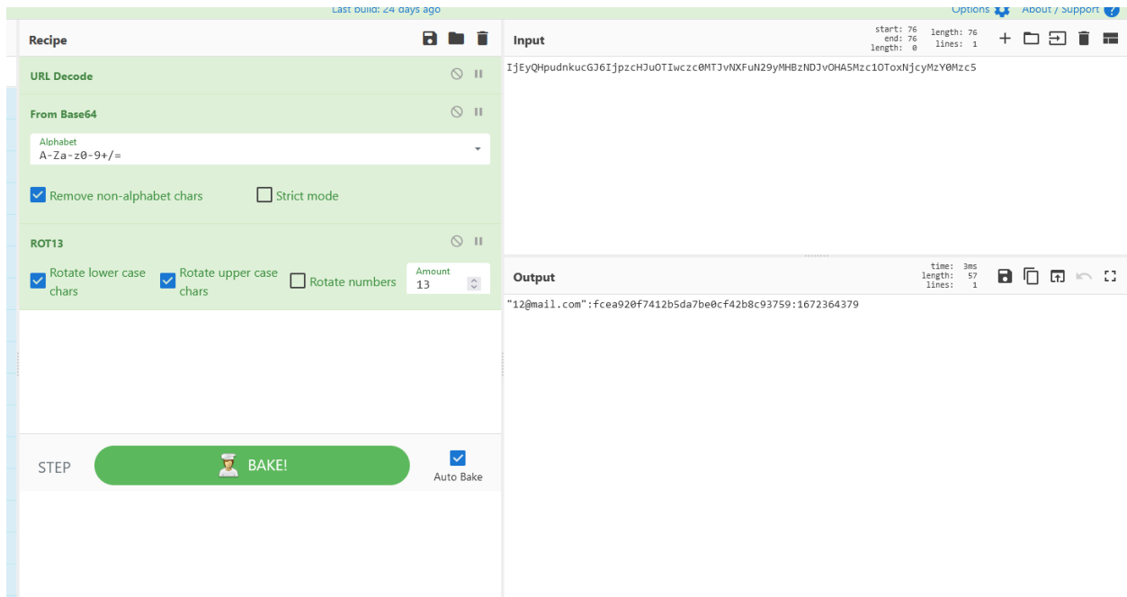
Figure 52 Cyber Chef
