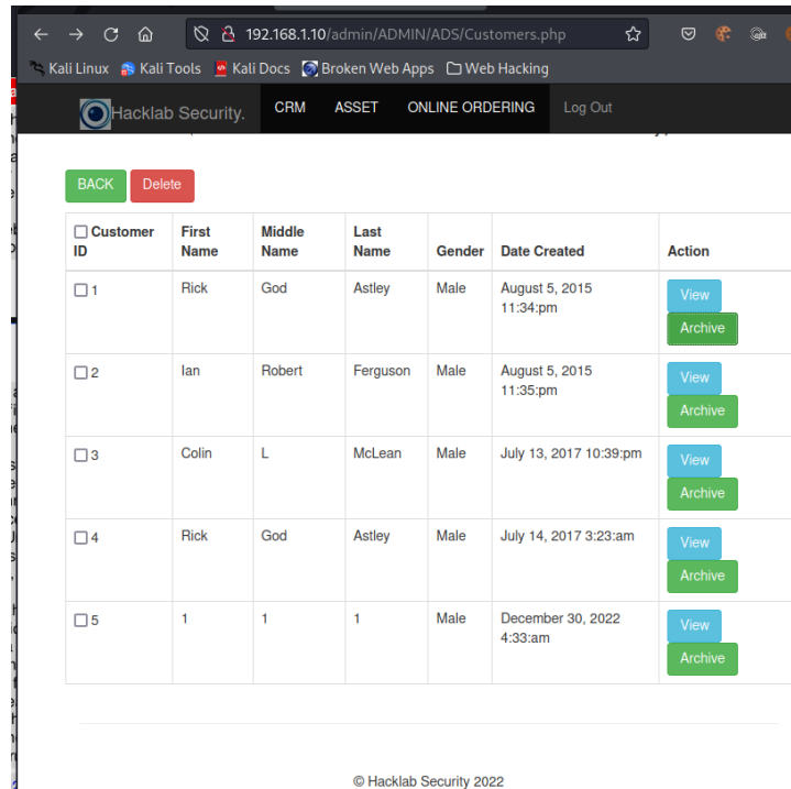
Figure 48 Customers.php
