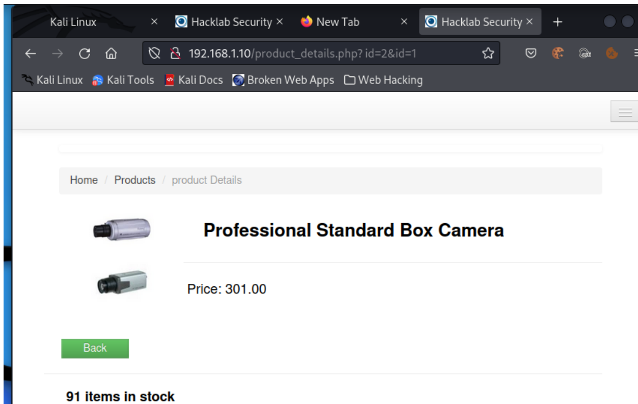
Figure 51 'product_details.php'
