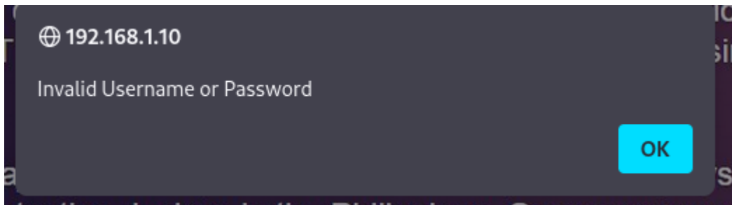
Figure 33 Incorrect username/password
