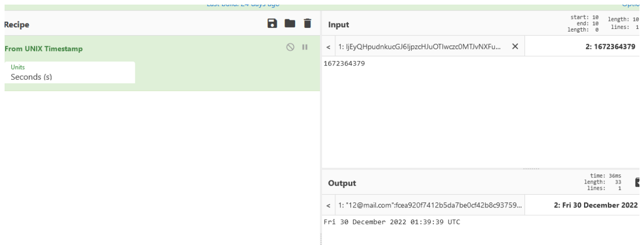
Figure 55 Unix timestamp
