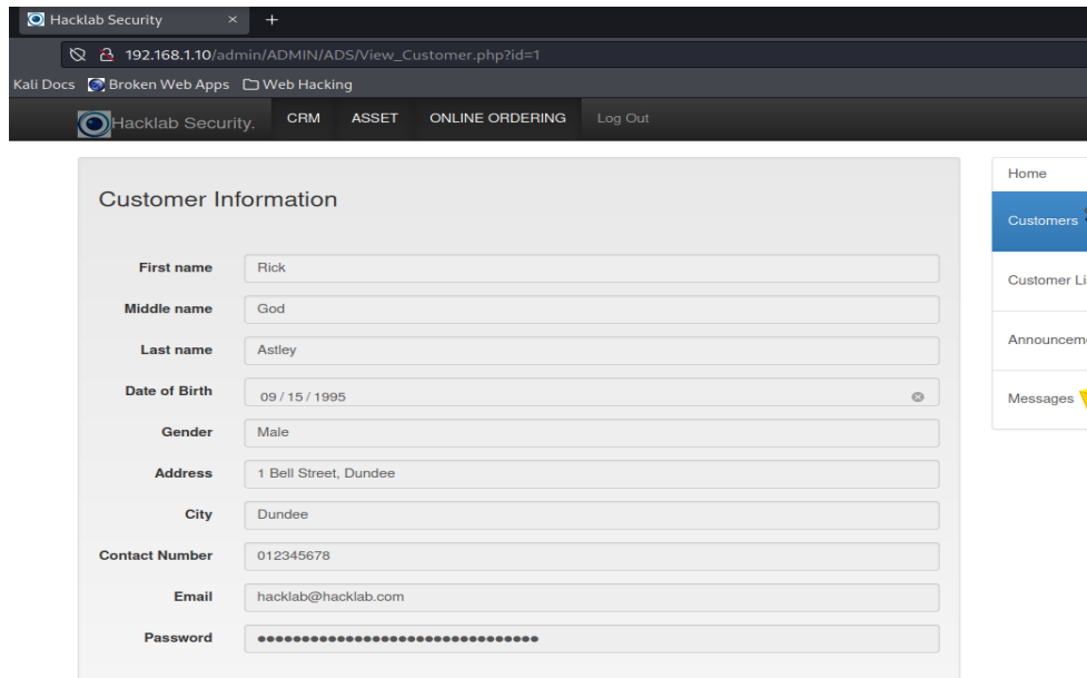
Figure 41 Customer Information
