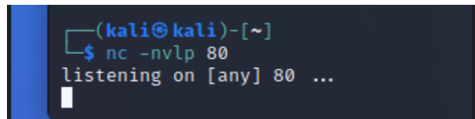
Figure 61 netcat listener
