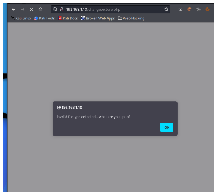
Figure 66 test.php upload
