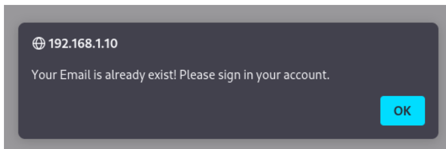
Figure 36 user credentials
