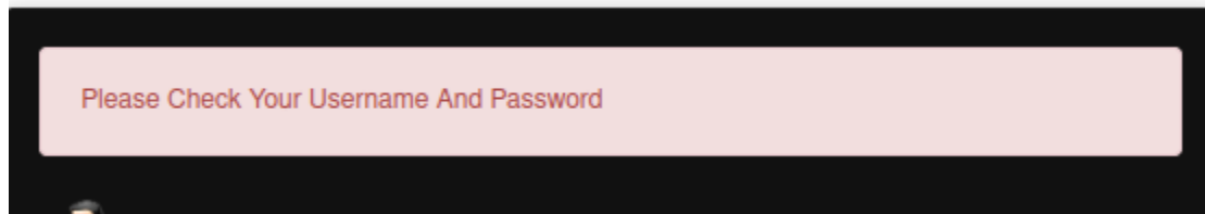
Figure 39 Incorrect credentials
