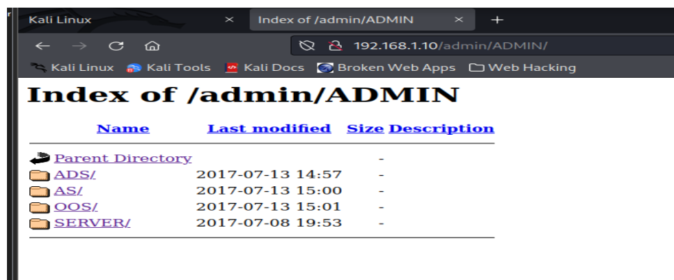
Figure 40 Admin Directory
