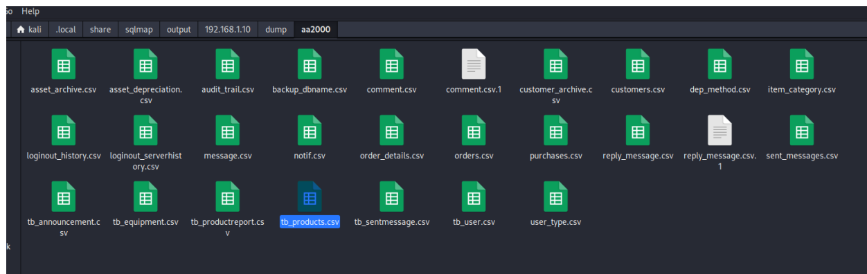
Figure 64 SQLMAP output
