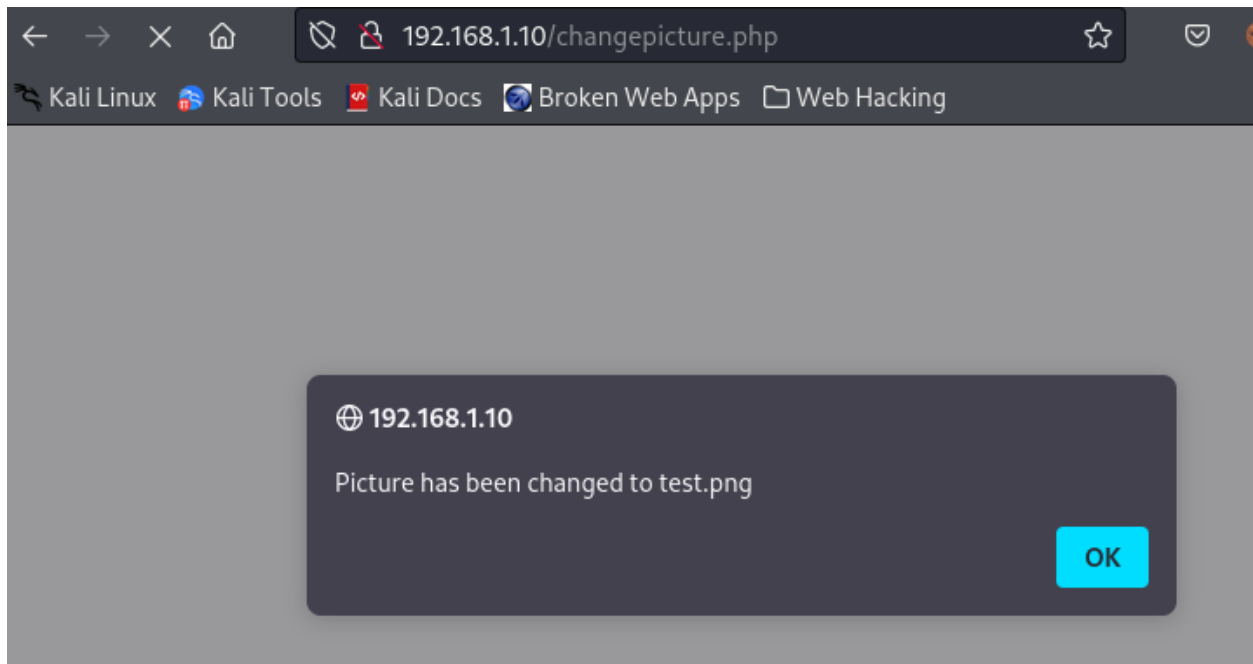
Figure 67 Change picture
