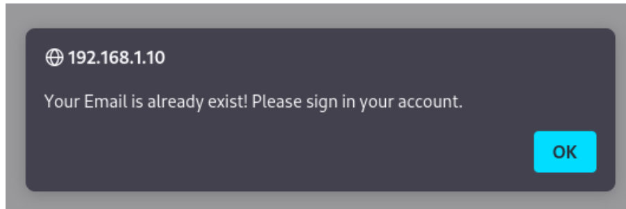
Figure 30 Pre-used email
