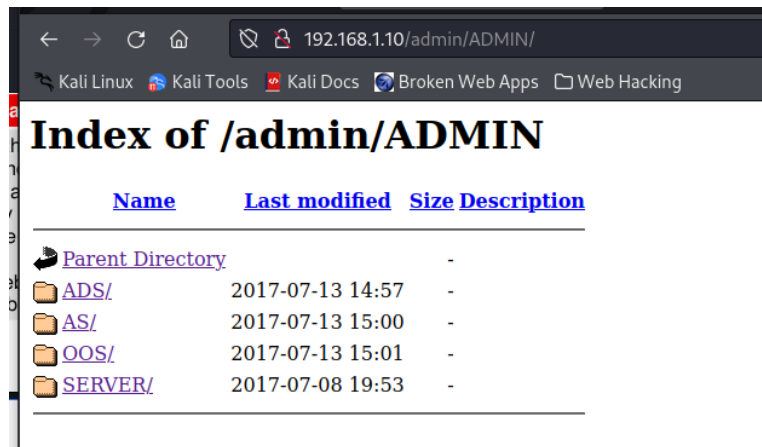
Figure 46 Admin directory
