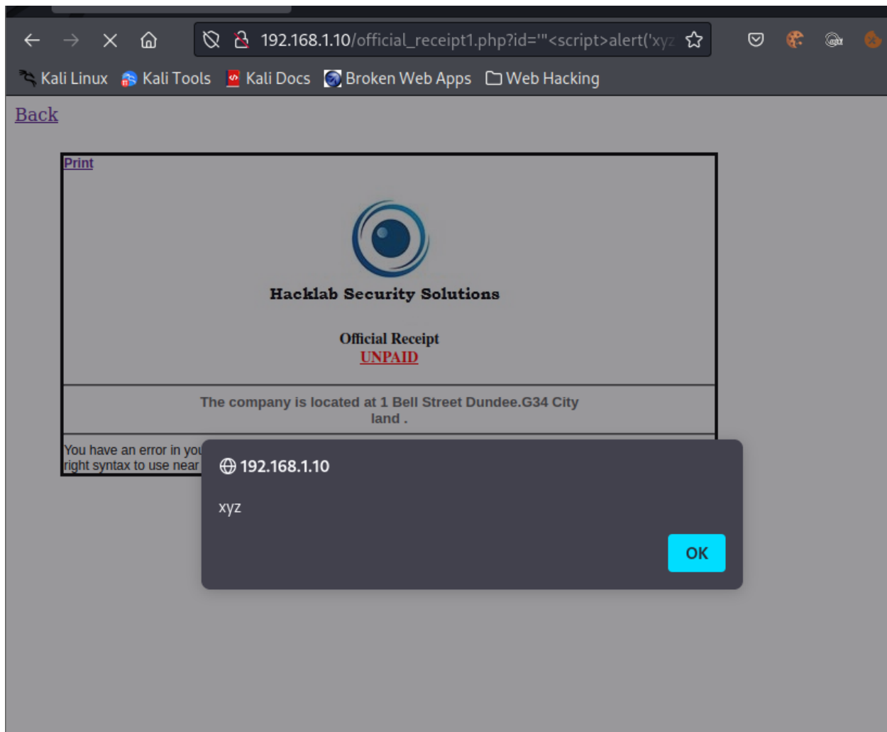
Figure 59 Reflected XSS
