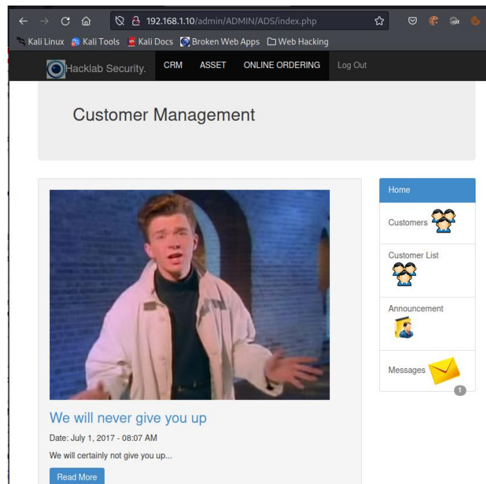
Figure 47 index.php
