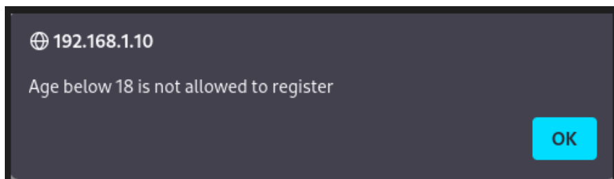
Figure 28 18+ error message
